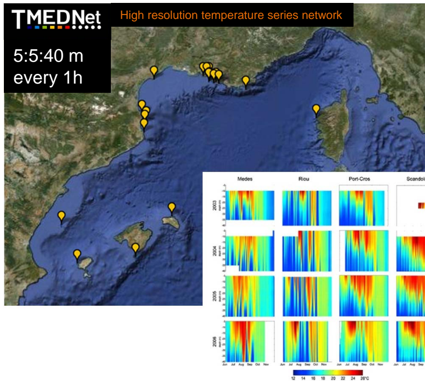
Fig. 5. Time series of daily mean T from June to November for 2003 to 2006 at Medes, Riou, Port-Cros, and Scandola.
